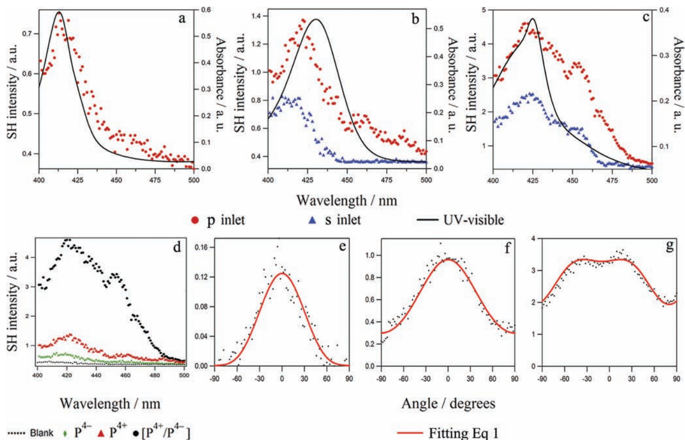
Figure 3. SSHG spectra of 100 \mu\text{M} of (a) P 4+ , CoTPPS 4+ ; (b) P 4+ , CoTMPyP 4+ ; (c) [P 4+ /P 4- ], equimolar mixture of both porphyrins; (d) comparison between the SSHG spectrum of the three systems. Polarization angle dependence of the fundamental beam on the SSHG intensity for (e) P 4- ; (f) P 4+ ; (g) [P 4+ /P 4- ].
